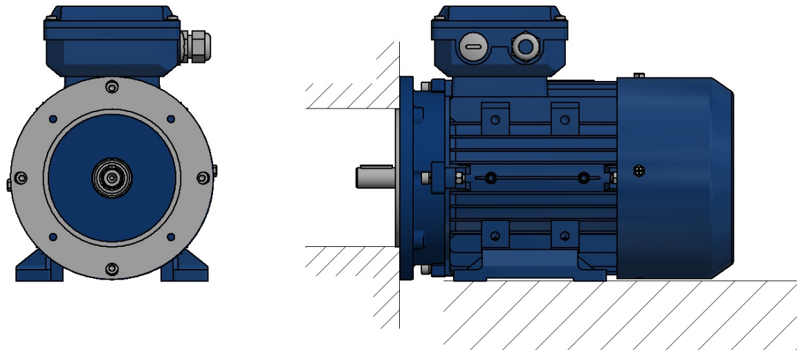
B34L (B3 and B14L) Foot and Large C-face flange mounted motor
